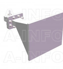
LB-137-15-C-TFSPO Standard Gain Horn Antenna 5.85-8.2GHz 15dB Gain TNC Female
