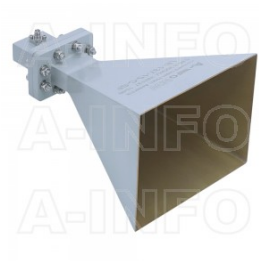
LB-137-15-C-SF Standard Gain Horn Antenna 5.85-8.2GHz 15dB Gain SMA Female
