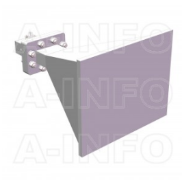
LB-137-15-C-SFSPO Standard Gain Horn Antenna 5.85-8.2GHz 15dB Gain SMA Female
