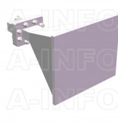
LB-137-15-C-3.5SFSPO Standard Gain Horn Antenna 5.85-8.2GHz 15dB Gain 3.5mm Female
